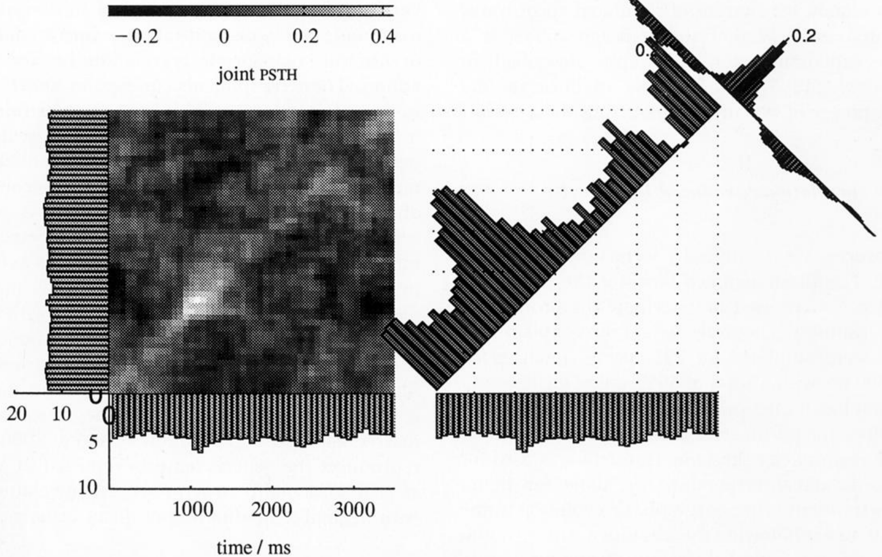
Figure 2. Joint peri-stimulus time histogram (JPSTH) based on the simulated data described in figure 1. The simulated spike trains were time-averaged in bins of 70 ms and subject to JPSTH analysis. The results of this analysis are seen above and should be compared with figure 2a in Vaadia et al. Left: mean firing rate (per second) averaged over epochs (side panels). These data correspond to a conventional peri-stimulus time histogram (PSTH) and show little modulation when referred to the stimulus events. The main panel is an image representation of the cross-correlation matrix (referred to the stimulus event at 1000 ms). Right: coincidence-time histogram (main diagonal) showing the time-dependent nature of the correlations (referred to the stimulus event) and conventional time-averaged cross-correlogram (upper right).
